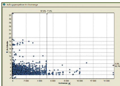
Scatter Chart
