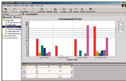
Bar Chart
