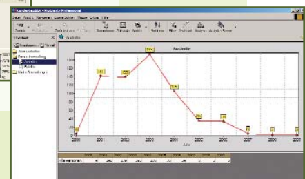
Line Graph
